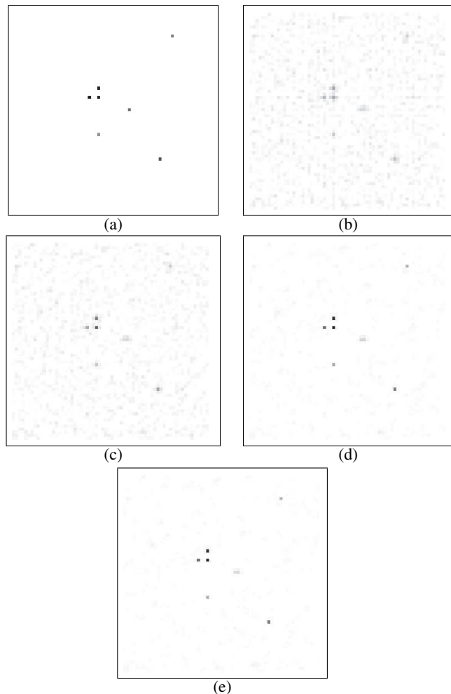
Fig. 2. Images are presented with the same inversed grayscale: (a) true image of 7 peaks, (b) FBP with ramp filter, (c) MCMC Gibbs approach, (d) classical variational Bayesian, (e) our method.
