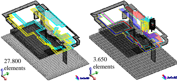
Fig. 2. Capacitive (left) and inductive (right) meshes - InCa3D [5]
