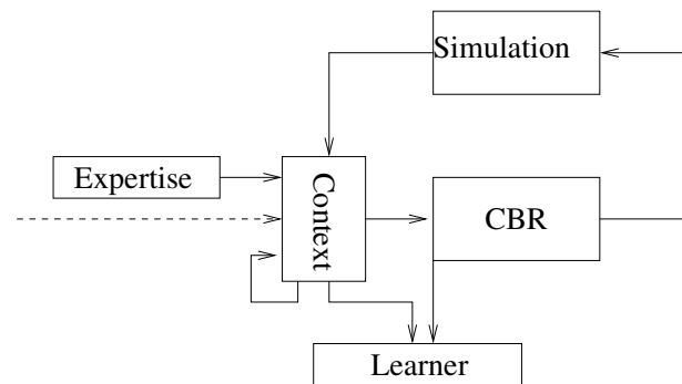
Figure 1: context division
