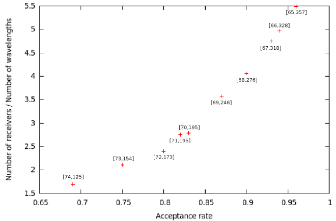
Fig. 1. Influence of the acceptance rate \tau on [z, W]
