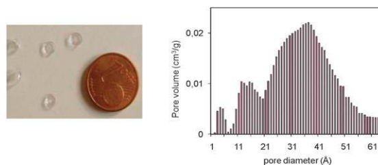
Fig. 4 Left: Mesoporous monolithic and transparent disks for the reversible trapping of aromatic monocyclic hydrocarbons. Right: Distribution of micro- and mesopores obtained from the analysis of the BET adsorption-desorption isotherms using the differential functional theory model.
