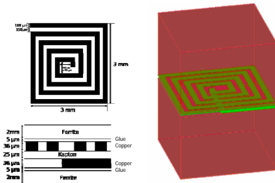
Fig. 8. Micro-inductance, composed by two magnetic regions ( \mu_r = 1000 ) and an electric inductance powered by a source voltage ( V = 1 volt, f = 1 kHz).
