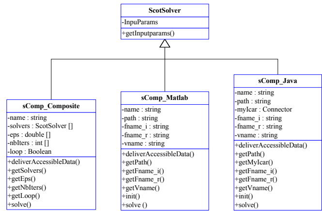
Fig. 5. Simplified UML diagram of the ScotSolver class and its subclasses.
