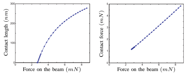
Fig. 2. Results of the semi-analytical structural contact model
