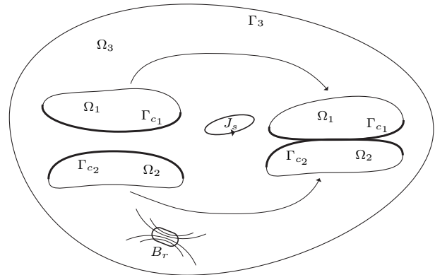
Fig. 1. Study domain of magneto-mechanical contact problem ( \Omega = \Omega_m \cup \Omega_3 and \Omega_m = \Omega_1 \cup \Omega_2 )
