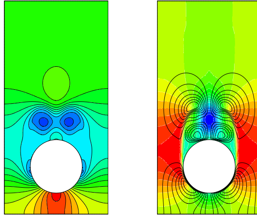
Fig. 2 ACF11-ball with (VPP _{\varepsilon} ) method, \varepsilon = 10^{-6} : free fall of a heavy solid body in air at time t = 0.15 and \text{Re} = 7358 - Cylinder diameter \varnothing = 0.05 , \rho_s = 10^6 , \rho_f = 1 , \mu_s = 10^{12} , \mu_f = 10^{-5} , domain 0.1 \times 0.2 , mesh size 256 \times 512 , \delta t = 0.0002 , cylinder initially with no motion at height y = 0.15 . LEFT: isobars and isoline \varphi = 0.5 of the phase function at interface. RIGHT: vertical velocity field and horizontal velocity isolines.
