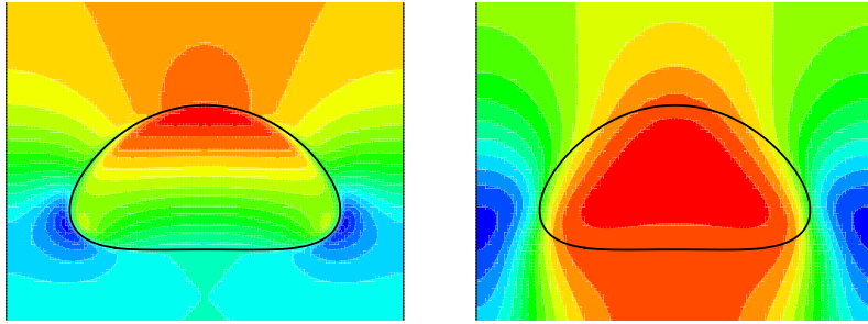
Fig. 1 Benchmark for 2-D bubble dynamics with (VPP_\varepsilon) method, \varepsilon = 10^{-8} : motion of a circular bubble with surface tension at time t = 3 and Re = 35 - bubble initial diameter \varnothing = 0.05 , \rho_1/\rho_2 = 1000/100 = 10 , \mu_1/\mu_2 = 10/1 = 10 , domain 0.1 \times 0.2 , mesh size 128 \times 256 , \delta t = 0.007143 , circular bubble initially with no motion at height y = 0.05 . LEFT: isobars and isoline \varphi = 0.5 of the phase function at interface. RIGHT: superposition of isoline \varphi = 0.5 at interface for (UAL), (SIP), (VPP) and vertical velocity field (in absolute referential).
