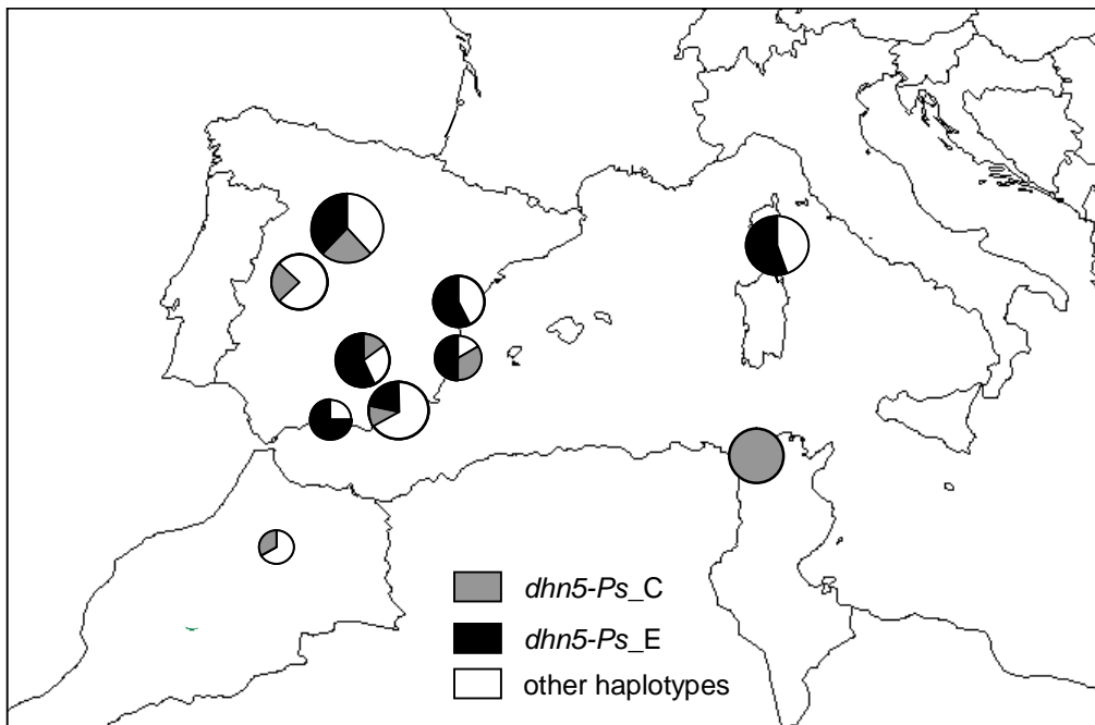
Figure 3. Upper section: dhn5 - Ps haplotype distribution showing the proportion of haplotypes C (in grey), E (in black) and all others (in white) in P. pinaster . The size of the pie is proportional to the sample size at each location. Lower section: expected (sigmoid curves) and observed covariation in haplotype frequencies of dhn5 - Ps _C and dhn5 - Ps _E and climatic variables. Expected curves were obtained under a logistic regression model including a single environmental variable (AMT or MTWM) after controlling for neutral processes (i.e. using the PCs of neutral molecular markers as covariates) for P. pinaster . AMT: annual mean temperature; MTWM: maximum temperature of the warmest month.
