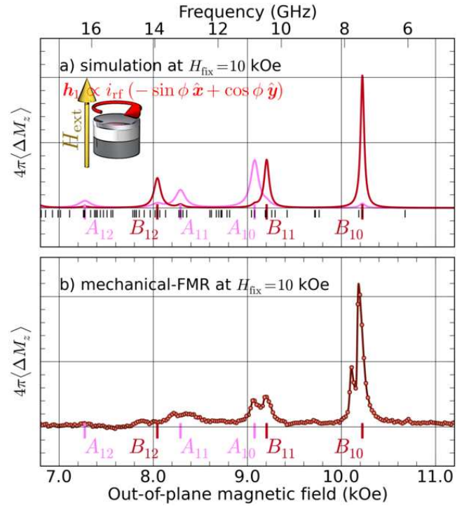
FIG. 10. (Color online) Panel (a) is the simulated spectral response to an orthoradial excitation field \mathbf{h}_1 \propto -\sin\phi\hat{x} + \cos\phi\hat{y} . Panel (b) recalls the experimental spectrum measured by mechanical-FMR for an RF current excitation.
