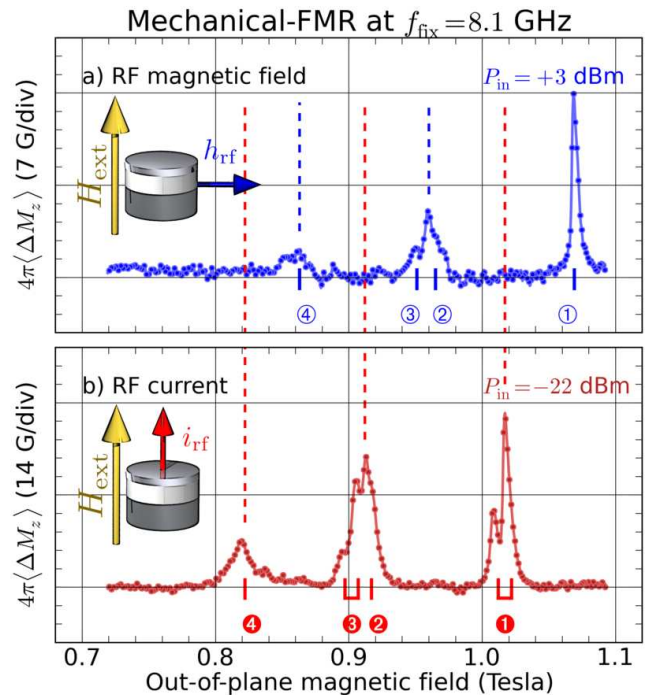
FIG. 2. (Color online) Comparative spectroscopic study performed by mechanical-FMR at f_{\text{fix}} = 8.1 \text{ GHz} , demonstrating that distinct spin-wave spectra are excited by a uniform in-plane RF magnetic field (a) and by an RF current flowing perpendicularly through the layers (b). The positions of the peaks are reported in Table II.
