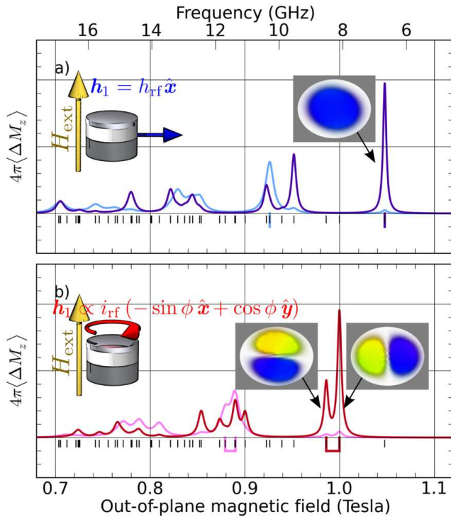
FIG. 13. (Color online) Simulated SW spectra for a nano-pillar with an elliptical section (see text). The panel (a) shows the linear response to a homogeneous RF magnetic field excitation and (b) to an orthoradial Oersted field excitation. The precession patterns of the lowest energy modes are shown in the insets.
