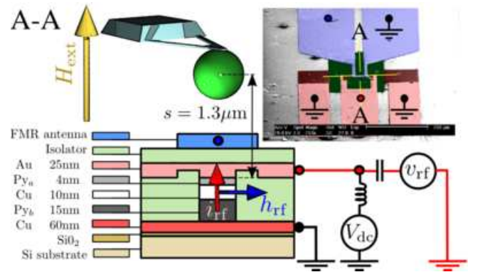
FIG. 1. (Color online) Schematic representation of the experimental setup used for this comparative spin-wave spectroscopic study. The magnetic sample is a circular nano-pillar comprising a thin (label a ) and a thick (label b ) magnetic layers separated by a normal metal spacer. It is saturated by a large magnetic field \mathbf{H}_{\text{ext}} applied along its normal axis. A Magnetic Resonance Force Microscope monitors the incoherent part of the forced oscillation regime inside the buried structure. The inset is a top view image of the two independent excitation circuits: in red the circuit allowing the injection of an RF current perpendicular-to-plane through the nano-pillar ( i_{\text{rf}} , red arrow); in blue the circuit allowing the generation of an RF in-plane magnetic field ( h_{\text{rf}} , blue arrow). The nano-pillar is at the center of the yellow cross-hair. The main figure is a section along the A - A direction.
