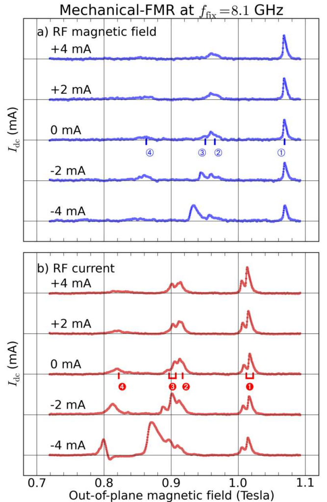
FIG. 3. (Color online) Evolution of the SW spectra measured at f_{\text{fix}} = 8.1 GHz by mechanical-FMR for different values of the continuous current I_{dc} flowing through the nano-pillar. The panel (a) corresponds to excitation by a uniform RF magnetic field (as in FIG. 2a), and the panel (b) to excitation by an RF current through the sample (as in FIG. 2b).
