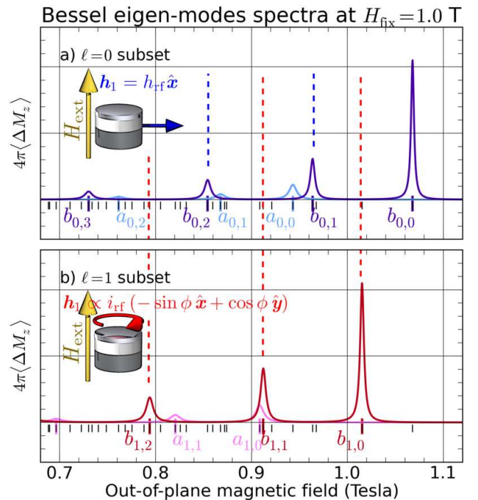
FIG. 7. (Color online) Analytically calculated spectra at H_{\text{fix}} = 1.0 T using the set of Bessel functions (see FIG.6) as the trial eigen-vectors. The panel (a) shows the linear response to an uniform excitation field \mathbf{h}_1 \propto \hat{x} and the panel (b) shows the linear response to an orthoradial excitation field \mathbf{h}_1 \propto -\sin \phi \hat{x} + \cos \phi \hat{y} . A light (dark) color is used to indicate the energy stored (cf. Eq.(12)) in the thin (thick) layer.
