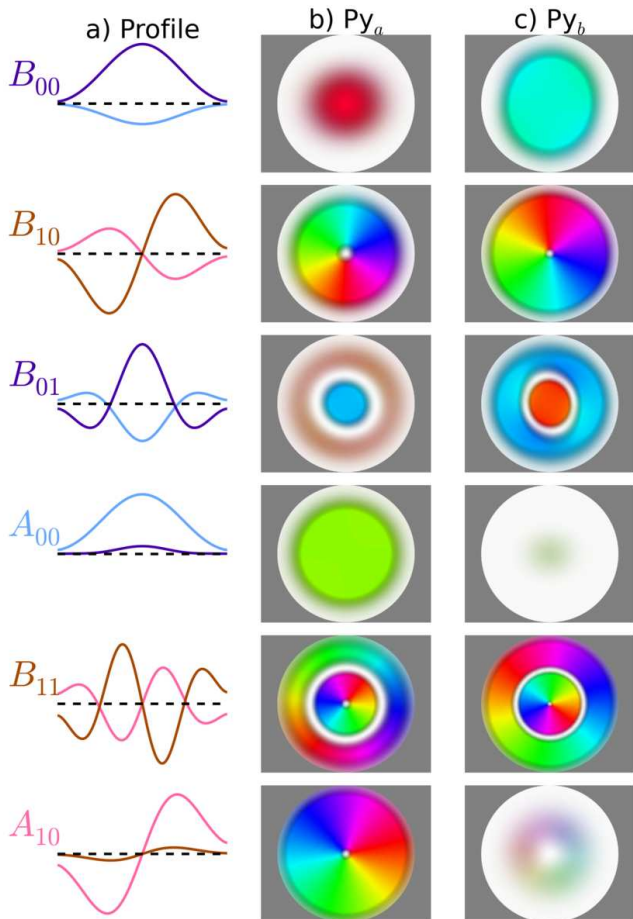
FIG. 11. (Color online) Simulated precession patterns of the eigen-vectors. Column (a) shows the precession profiles across the thin (light color) and thick (dark color) layers. Columns (b) and (c) show the dynamics in the thin \text{Py}_a and thick \text{Py}_b layers, respectively, with the color code defined in FIG. 6.
