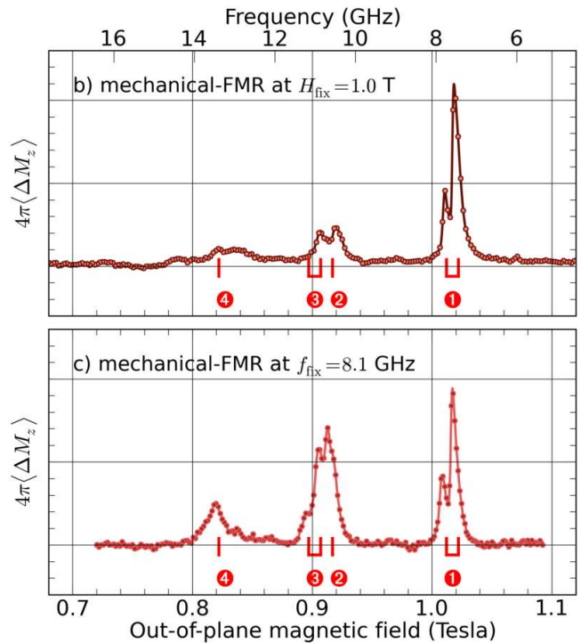
FIG. 4. (Color online) Frequency-field dispersion relation: the top spectrum is measured at constant bias field H_{\text{fix}} = 1 \text{ T} by sweeping the frequency of the RF current i_{\text{rf}} through the nano-pillar. The bottom spectrum is the same as in FIG.2b, i.e. , it is obtained by sweeping the magnetic field at fixed frequency f_{\text{fix}} = 8.1 \text{ GHz} of i_{\text{rf}} . The top and bottom scale are in correspondence through the affine transformation H_{\text{ext}} - H_{\text{fix}} = 2\pi(f - f_{\text{fix}})/\gamma .
