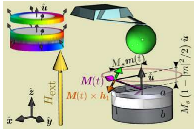
FIG. 5. (Color online) Schematic representation of the magnetization dynamics under continuous RF excitation. In the steady state, the torque exerted by the perturbation RF excitation field \mathbf{h}_1 (orange arrow) compensates the torque exerted by the damping (green), and the local magnetization vector \mathbf{M}(t) (purple) precesses at the Larmor frequency on a circular orbit around the local equilibrium direction (unit vector \hat{\mathbf{u}} ). \mathbf{M}(t) is the sum of a small oscillating component M_s \mathbf{m} and a large static component M_s (1 - |\mathbf{m}|^2/2) , respectively transverse and parallel to \hat{\mathbf{u}} . The inset shows the simulated spatial distribution of \hat{\mathbf{u}} inside the nano-pillar at \mathbf{H}_{\text{ext}} = 1.0 T (see section IV C). In the white regions, the magnetization is aligned along the normal \hat{\mathbf{z}} within 0.05^\circ . In the colored regions, \hat{\mathbf{z}} is flaring ( < 5^\circ ) in the radial direction (the hue indicating the direction of \hat{\mathbf{u}} - \hat{\mathbf{z}} , according to the color code defined in FIG. 6).
