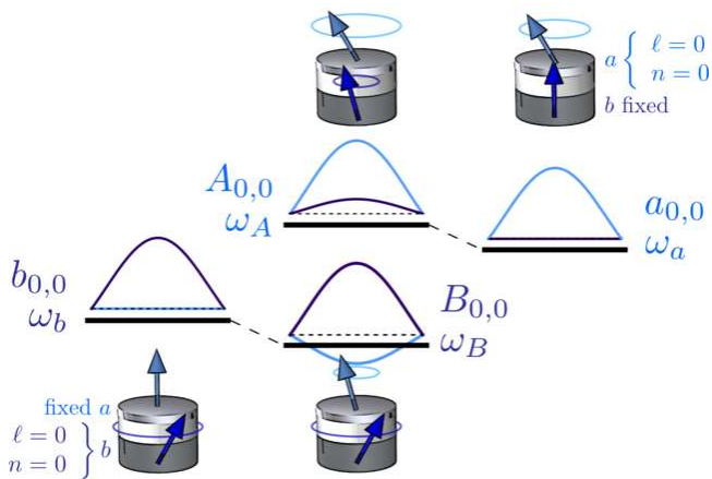
FIG. 8. (Color online) (a) Schematic representation of the coupled dynamics between two different magnetic disks. Here, \omega_b , the eigen-frequency of the lowest energy precession mode in the thick layer (the thin layer being fixed at equilibrium) is smaller than \omega_a , the one in the thin layer (the thick layer being fixed at equilibrium). When the two disks are dynamically coupled through the dipolar interaction, the binding state B corresponds to the two layers oscillating in anti-phase at \omega_B , with the precession occurring mostly in the thick layer, whereas the anti-binding state A corresponds to the layers oscillating in phase at \omega_A , with the precession mostly in the thin layer. This is shown by displaying the precession profile \mathbf{m}(\rho) in each layer using a light (dark) color to represent the contribution of the thin (thick) layer.
