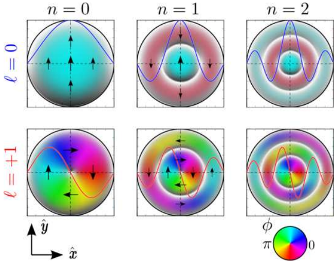
FIG. 6. (Color online) Color representation of the spatial pattern of the Bessel eigen-vectors for different values of the azimuthal mode index \ell (by row) and radial mode index n (by column). Arrows are a snapshot of \mathbf{m} in the disk. All arrows are rotating synchronously in-plane at the Larmor frequency. In our coding scheme, the hue indicates the phase \phi = \arg(\mathbf{m}) (or direction) of \mathbf{m} , while the brightness indicates the amplitude of |\mathbf{m}|^2 . The nodal positions (regions where there is no precession, |\mathbf{m}| = 0 ) are marked in white.
