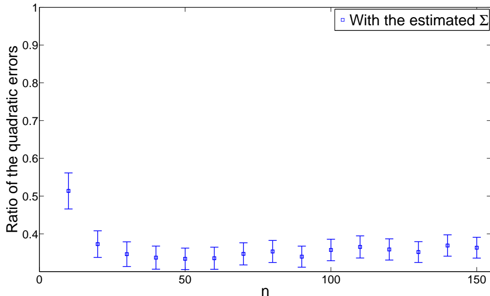
Figure 6: Increasing the sample size n (Experiment B), improvement of multi-task compared to single-task: \mathbb{E}[\|\hat{f}_{\text{similar}, \hat{\Sigma}} - f\|^2 / \|\hat{f}_{\text{ind}, \hat{\Sigma}} - f\|^2] .
