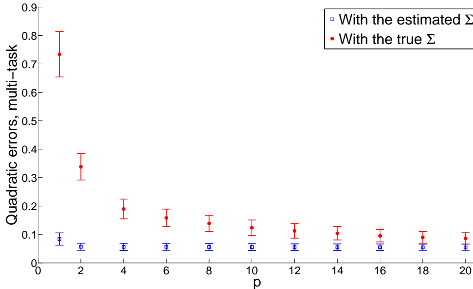
Figure 2: Increasing the number of tasks p (Experiment A), quadratic errors of multi-task estimators (np)^{-1}\mathbb{E}[\|\hat{f}_{\text{similar},S} - f\|^2] . Blue: S = \hat{\Sigma} . Red: S = \Sigma .
