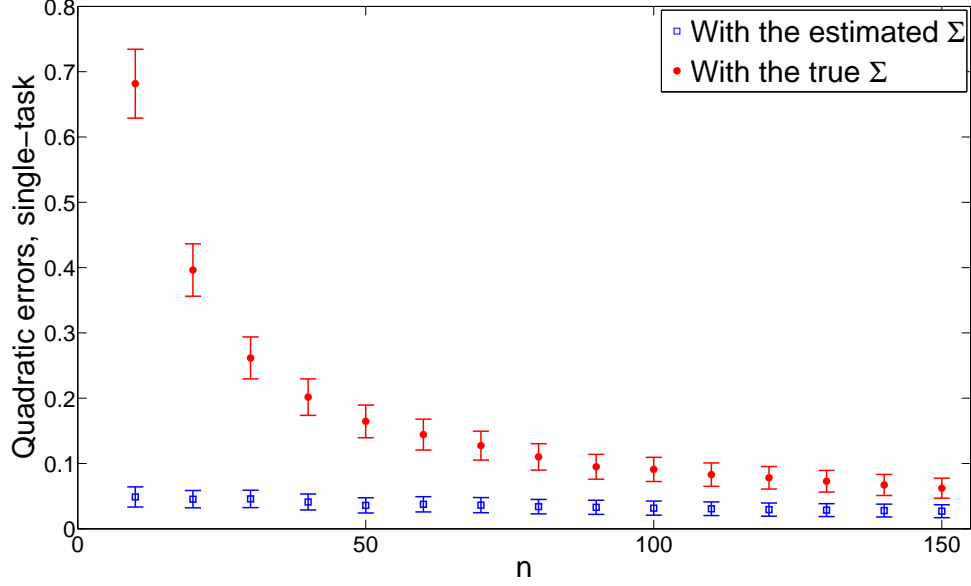
Figure 5: Increasing the sample size n (Experiment B), quadratic errors of single-task estimators (np)^{-1}\mathbb{E}[\|f_{\text{ind},S} - f\|^2] . Blue: S = \widehat{\Sigma} . Red: S = \Sigma .
