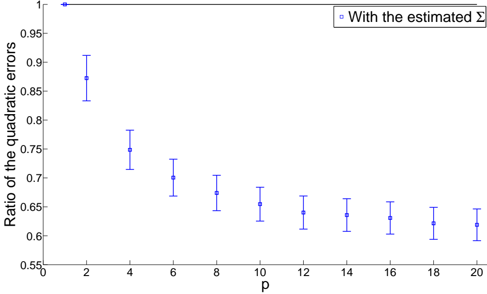
Figure 1: Increasing the number of tasks p (Experiment A), improvement of multi-task compared to single-task: \mathbb{E}[\|\widehat{f}_{\text{similar},\widehat{\Sigma}} - f\|^2 / \|\widehat{f}_{\text{ind},\widehat{\Sigma}} - f\|^2] .
