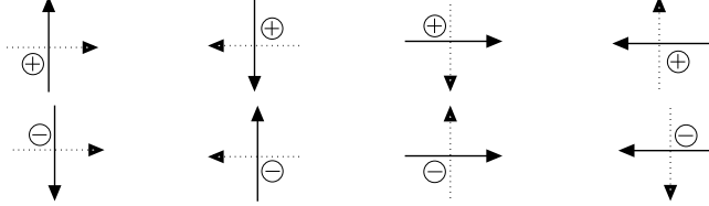
FIG. 4: All possible values of the orientations o_{\eta\gamma} of the crossing appearing in equation (21). The edges \eta regulating the flux operators are the dotted lines while the holonomies are along the continue lines \gamma .
