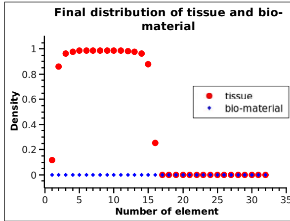
Figure 3. Equilibrium configuration of bone tissue and artificial material mass density for a low value of the applied external forces ( \tilde{F}^{ext} = 1 )
