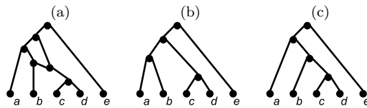
Fig. 1 (a) A level-1 network N . (b) and (c) The phylogenetic trees that form the tree system \mathcal{T}(N) .
