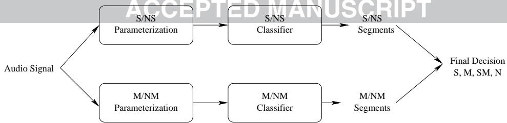
FIG. 5 – Architecture of our speech/music discrimination system.
