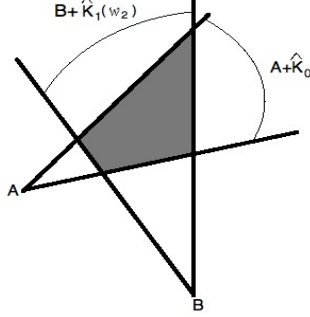
FIG 2. The grey-coloured domain corresponds to the set \Lambda := (\mathcal{F}_0, \hat{K}_1)\text{-Esssup} \{\hat{V}_1\} where \hat{V}_1 = AI_{\{\omega_1\}} + BI_{\{\omega_2\}} .
