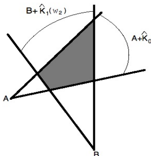
FIG 2. The grey-coloured domain corresponds to the set \Lambda := (\mathcal{F}_0, \hat{K}_1) -Esssup \{\hat{V}_1\} where \hat{V}_1 = AI_{\{\omega_1\}} + BI_{\{\omega_2\}} .
