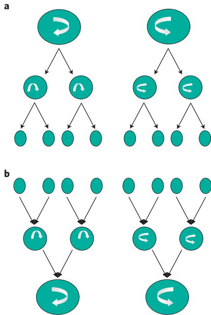
Figure 1 | Downscale and upscale energy transfers. a. In three dimensions, big eddies break up into smaller and smaller eddies. b. In two dimensions the small eddies give rise to larger and larger eddies.
