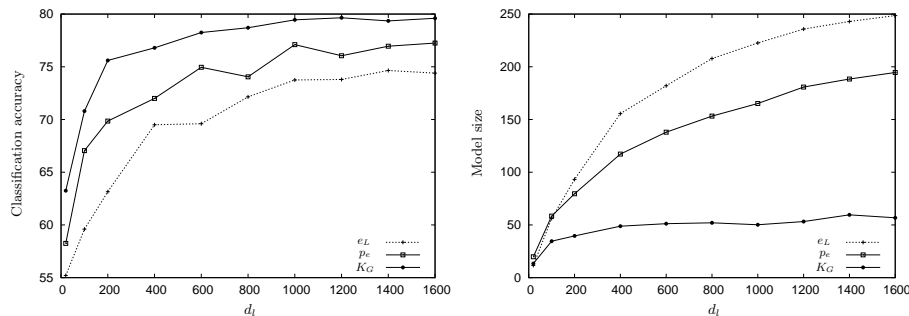
Fig. 2. Learning the separator: accuracy and sparsity results with respect to d_i .
