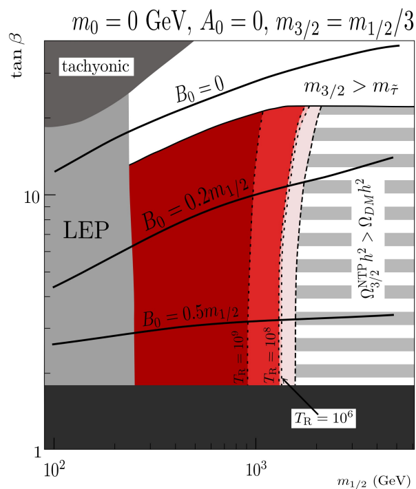
FIG. 10. Same as Fig 9 but for m_{3/2} = \frac{1}{3} m_{1/2} .
