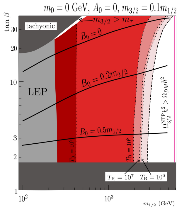
FIG. 9. Gravitino DM relic density values consistent with the WMAP constraints (5.8) in the (m_{1/2}, \tan \beta) plane, assuming m_{3/2} = 0.1 m_{1/2} and m_0 = A_0 = 0 . The different levels of red correspond to different reheating temperature values. The small region where the gravitino is not the LSP is also indicated; other captions as in Fig. 7.
