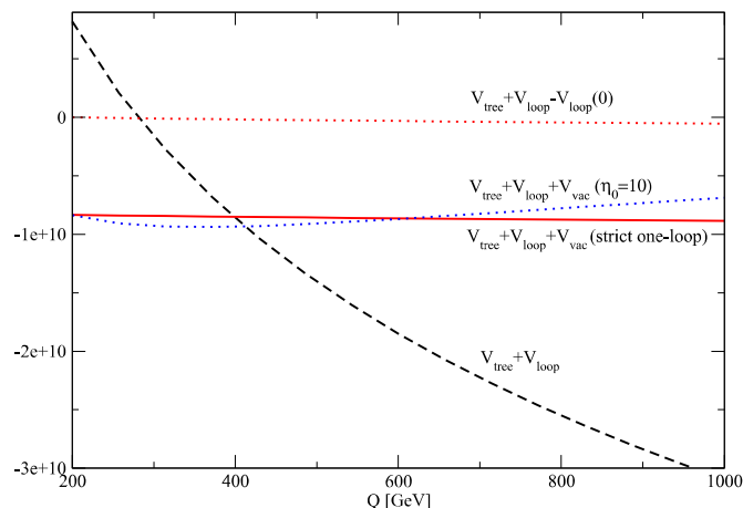
FIG. 1. The scale dependence of the effective potential, with or without the vacuum energy contributions, for representative input values B_0 = .2m_{1/2} , m_0 = A_0 = 0 , m_{1/2} = 300\text{GeV} and m_{top} = 173\text{ GeV} . Dashed line: without vacuum energy contribution; full line: V_{full} from Eq. (3.16) with running vacuum energy and \eta_0 = 10 at the strict one-loop order (i.e. no running of parameters inside one-loop expressions); dash-dotted line: same as the previous case but with all running parameters at one-loop, showing moderate spurious scale-dependence to be cancelled by two-loop contributions; dotted line: same with subtracted vacuum contribution from Eq. (3.15).
