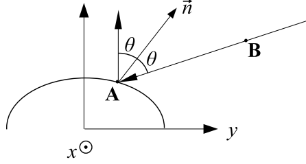
Figure 6: Description of the 3D-ray given by the points A and B .
