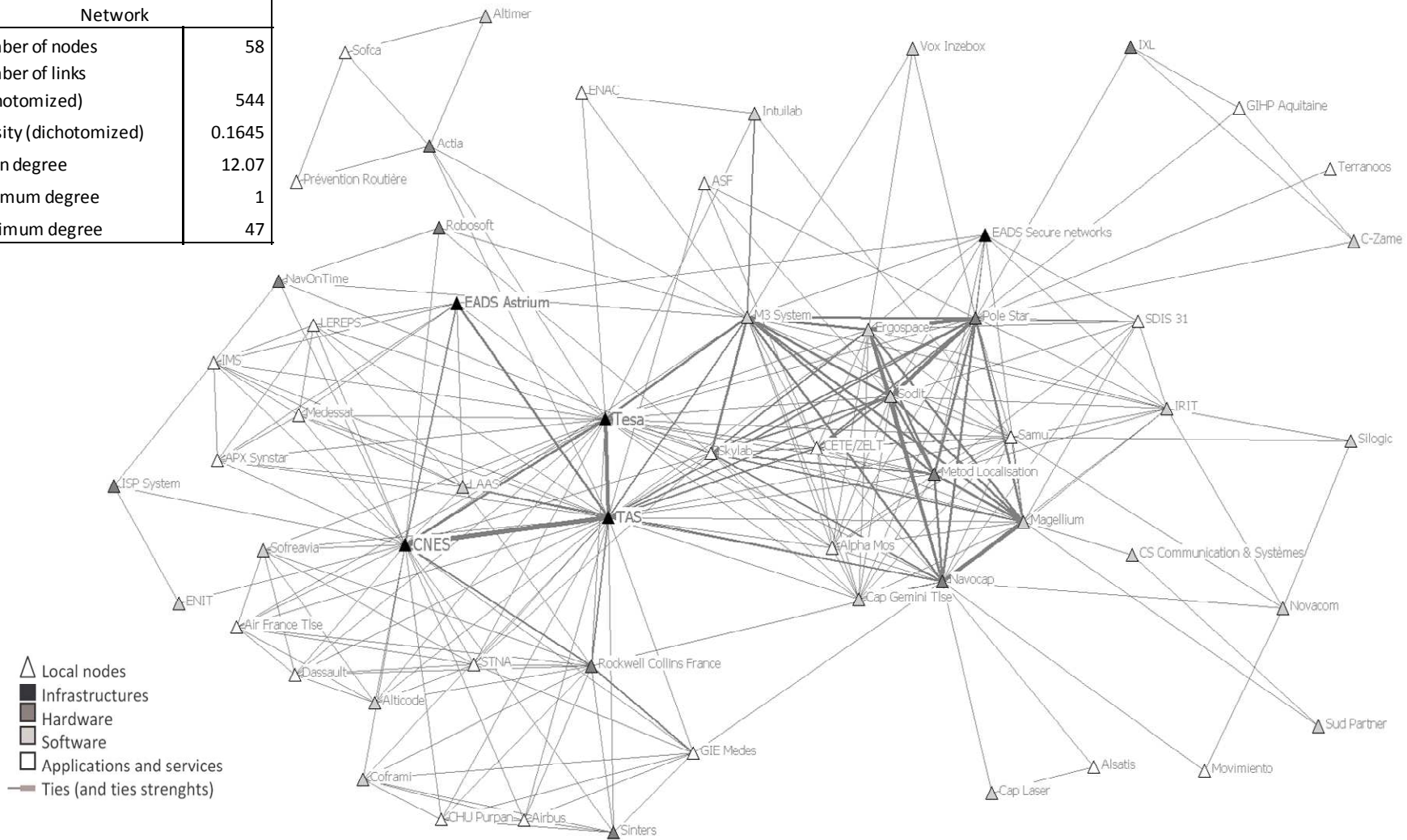
Figure 3: MP Network
