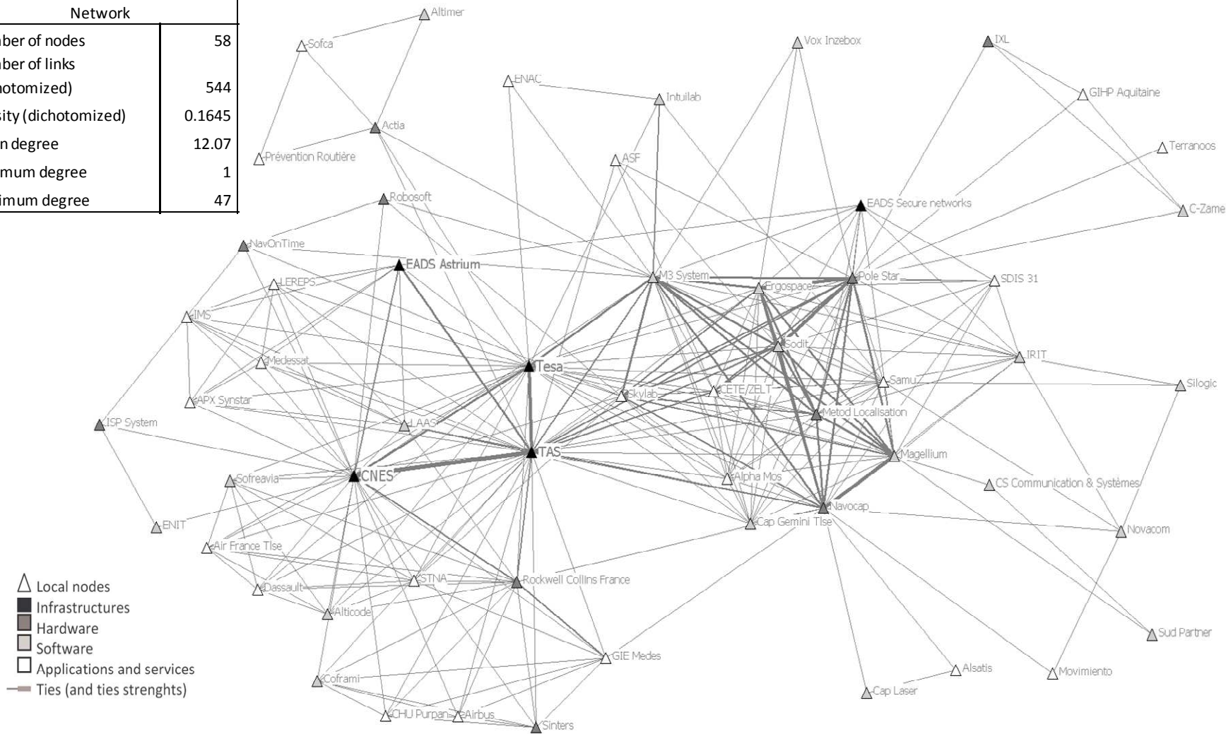
Figure 3: MP Network
