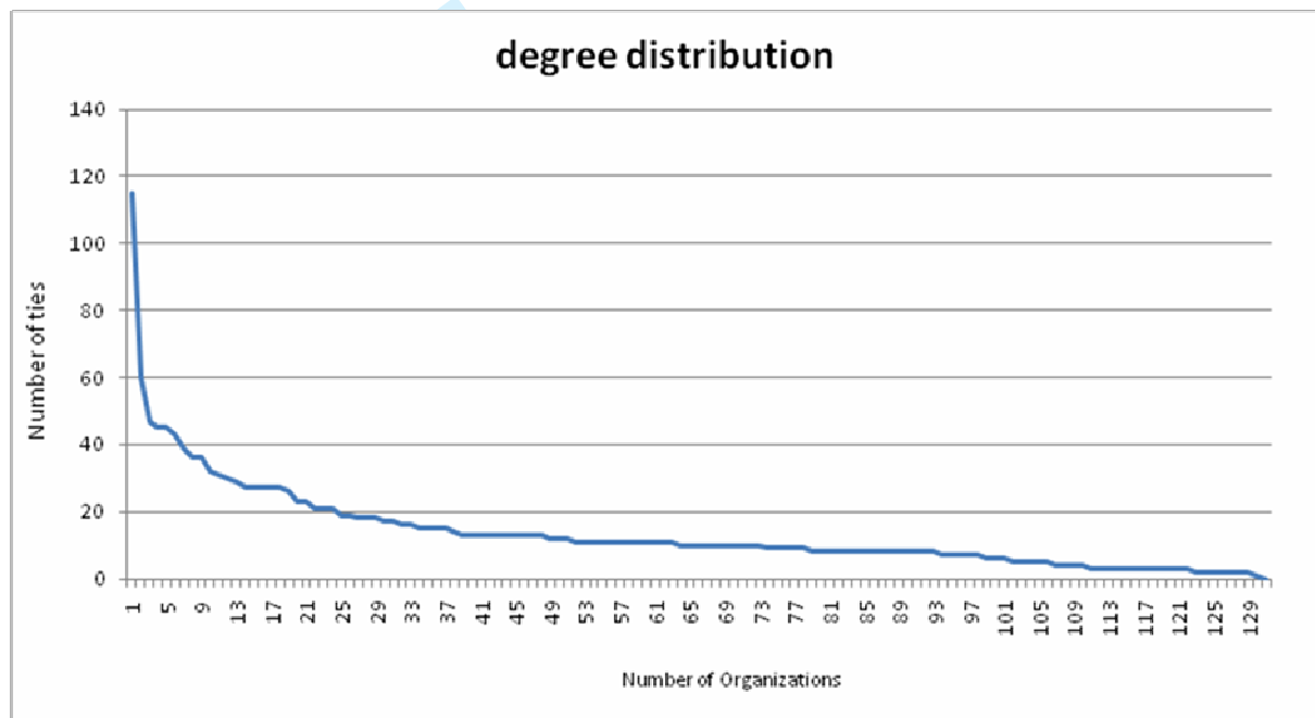
Figure 2: Degree distribution
