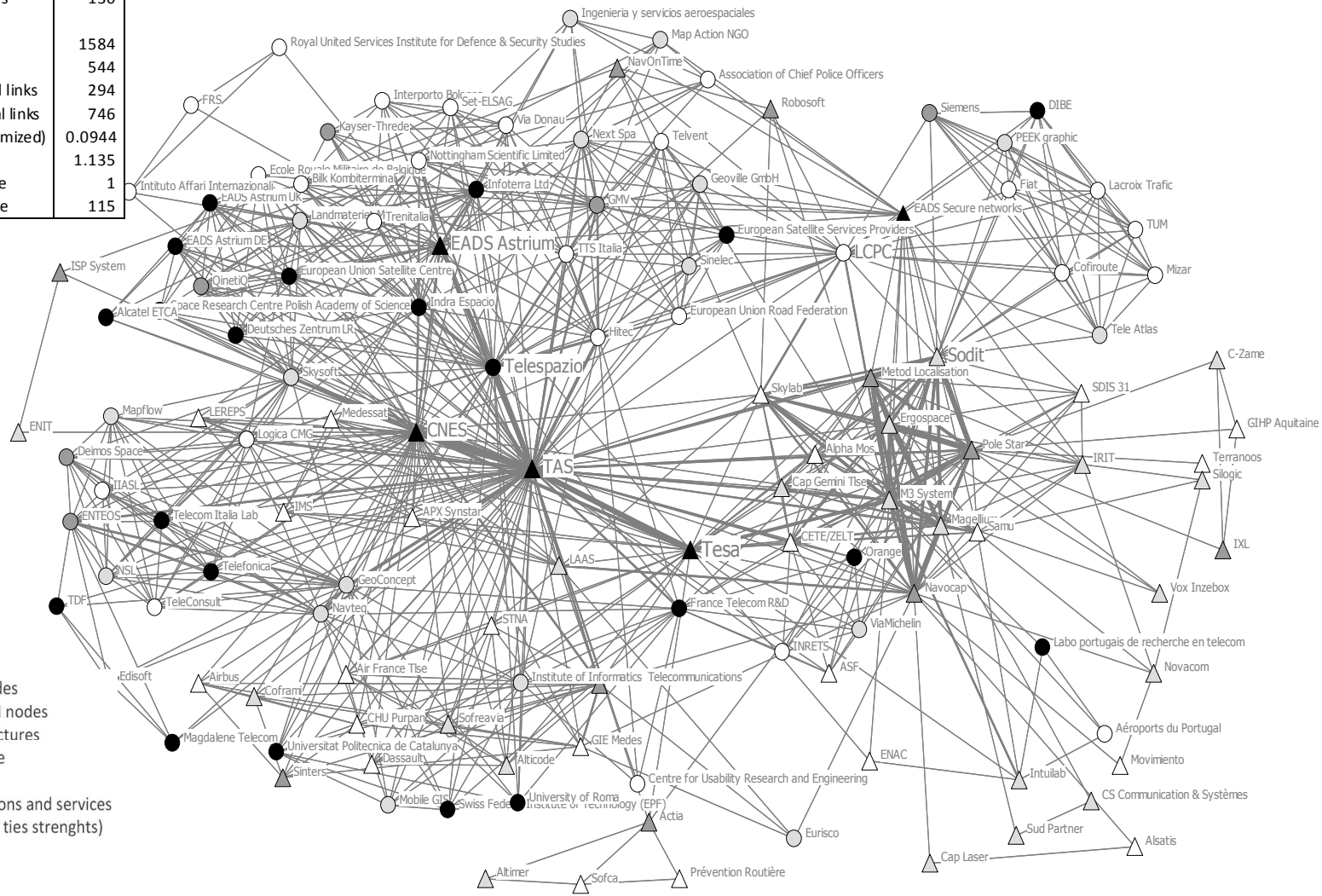
Figure 2: MP+ Network
