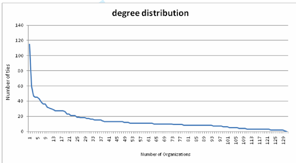
Figure 2: Degree distribution
