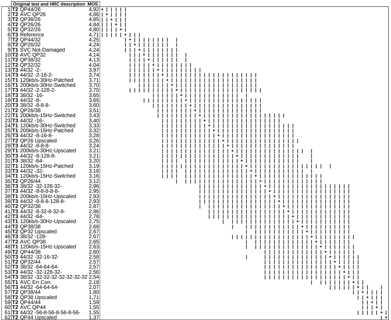
Figure 3: HRC comparison after mapping the results of T1 and T2 onto T3. Each HRC is marked with a '+' symbol. The '|' symbols denote the statistical equivalence between the MOS values of two HRCs.
