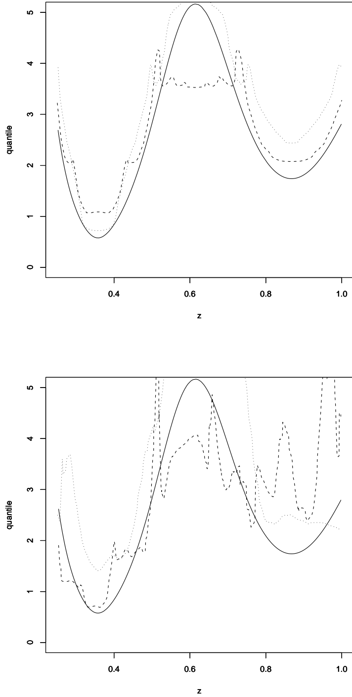
Figure 3: Comparison of the estimated quantile \hat{q}_n^w(\beta_n|x) corresponding to the median error with the true quantile function (continuous line). Horizontally: Z , vertically: quantiles. Two values of \alpha_n are considered: \alpha_n^{opt} (dashed line) and \alpha_n = 15 \log(n)/n (dotted line). Top: semi-metric d_Z , bottom: semi-metric d_X .
