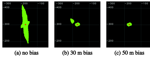
Fig. 9 Horizontal projection of the 1-relaxed solution with one biased measurement. Red dot is ground truth.
