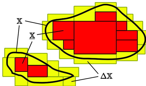
Fig. 3 Bracketing of the hatched set between two subpavings. Red boxes: inner subpaving \underline{\mathbf{X}} , Red and yellow: outer subpaving \overline{\mathbf{X}} = \underline{\mathbf{X}} \cup \Delta\mathbf{X}
