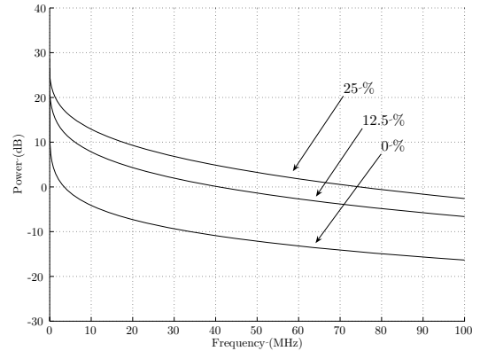
Fig. 6. Fitting curves with respect to the background noise model for a 30-meters cable.
