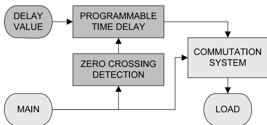
Fig. 3. Commutation tool.
