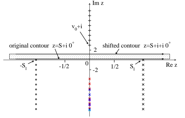
FIG. 1: (color online) In the complex plane, illustration of the procedure used to determine the Fourier transform of the function x \rightarrow e^x F^{(l)}(x) : Under the a posteriori checkable hypothesis (67) (no pole of \tilde{F}^{(l)}(z) in the grey area), one can shift the integration contour in (66) upwards by one unity along the vertical axis, to obtain the Fourier representation Eq. (68) of x \rightarrow e^x F^{(l)}(x) . Circles: Poles of \tilde{F}^{(l)}(z) due to the function hyperbolic sine in the denominator of (70). Pluses: Poles of \tilde{F}^{(l)}(z) due to the factors \Gamma(1+iz-iv_n) , n \geq 0 , in the numerators of the infinite product (73). Black crosses: Poles of \tilde{F}^{(l)}(z) due to the factor \Gamma(iS_l-iz) in (73). Colored crosses on the \text{Im } z < 0 part of the imaginary axis: Poles of \tilde{F}^{(l)}(z) due to the factors \Gamma(-iu_n-iz) for n > 0 in (73) [red: n=1 ; blue: n=2 ; violet: n=3 ; cyan: n=4 ]; from top to bottom, n=1 (three crosses), n=2 (two crosses), two triplets n=1, 2, 3 and a quadruplet n=1, 2, 3, 4 . The figure corresponds to l=1 and \alpha=20 .
