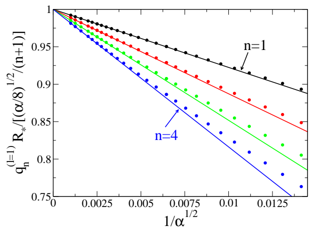
FIG. 8: (color online) Numerical study of the hydrogenoid part of the spectrum: For an angular momentum l = 1 , wavenumbers q_n^{(l)} for n = 1 (ground trimer state), n = 2 , n = 3 and n = 4 (from top to bottom), divided by the hydrogenoid asymptotic Born-Oppenheimer prediction (104), as functions of 1/\alpha^{1/2} . Disks: Numerical results. Straight lines: Asymptotic result (105) including the first deviation of the Born-Oppenheimer potential from the Coulomb form at short range. The color code is black for n = 1 , red for n = 2 , green for n = 3 and blue for n = 4 .
