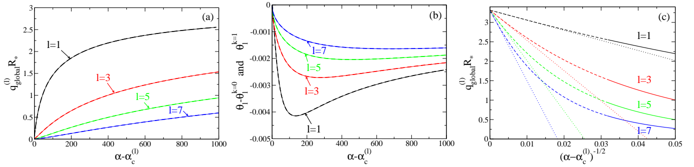
FIG. 4: (color online) In (a) value of the global wavenumber scale q_{\text{global}}^{(l)} of the Efimovian part of the spectrum, see (87), as a function of the difference of the mass ratio \alpha from its critical value, for all odd angular momenta up to l = 7 . Thin solid lines: Exact result obtained from (88) and from the infinite product representation (73) [the more rapidly converging form (C3,C5) was used in the numerics]. Thick dashed lines: Zeroth-order approximation omitting all the terms in the sum over k in (89). In (b) the (small) difference between the exact \theta_l and the zeroth-order approximation \theta_l^{k=0} is plotted as thin solid lines, and the value \theta_l^{k=1} of the k = 1 term of (89) is plotted as thick dashed lines. In (c) the values of q_{\text{global}}^{(l)} resulting from the Born-Oppenheimer plus semi-classical approximation are given in dashed lines [see Eq. (108)], as functions of 1/(\alpha - \alpha_c^{(l)})^{1/2} , showing how the l -independent \alpha \rightarrow +\infty limit is reached. The solid lines correspond to the exact numerical data of (a) and the dotted straight lines corresponds to the asymptotic expansion Eq. (110).
