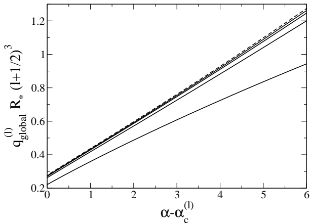
FIG. 5: Dependence, with the angular momentum l , of the global wavenumber scale q_{\text{global}}^{(l)} in the Efimov trimer spectrum, as obtained from the exact result (87). The figure shows the quantity q_{\text{global}}^{(l)} R_* multiplied by (l + 1/2)^3 , as a function of \alpha - \alpha_c^{(l)} , for (odd) angular momenta equal to l = 1 , l = 3 , l = 5 and l = 7 from bottom to top. This quantity is observed to converge rapidly to a finite limit for increasing l . The dashed line represents the analytical prediction (92) for that limit. We recall that E_{\text{global}} = -\hbar^2 q_{\text{global}}^2 / (2\mu) .
