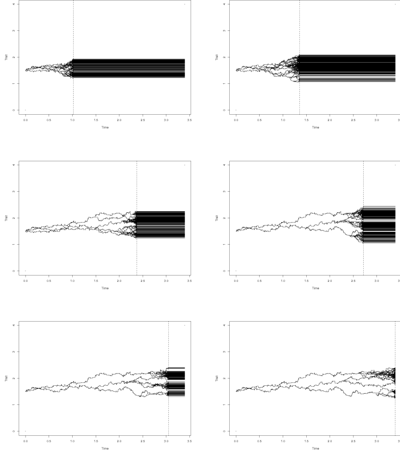
Figure 5: Kisdi's model . \alpha = 1.2 , \beta = 4 , x_0 = 4 , \sigma = 0.2 , p = 1 , K = 100 , n = 100 . The 100 particles are started with the trait 1.5.
