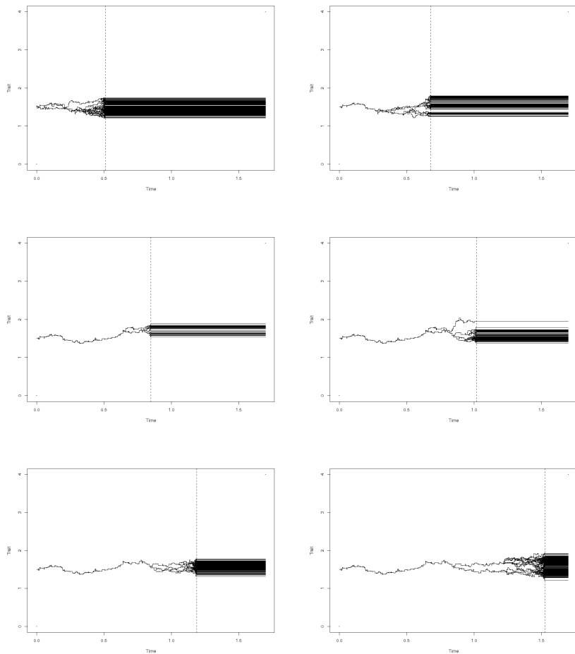
Figure 3: Dieckmann-Doebeli model . \sigma = 0.4 , \sigma_b = 0.4 , \sigma_U = 0.3 , x_0 = 4 , p = 0.5 , n = 300 . The 300 particles are started with the trait 1.5. In this example, \sigma_b > \sigma_U and we observe the separation of the population into two subgroups concentrated around different trait values.
