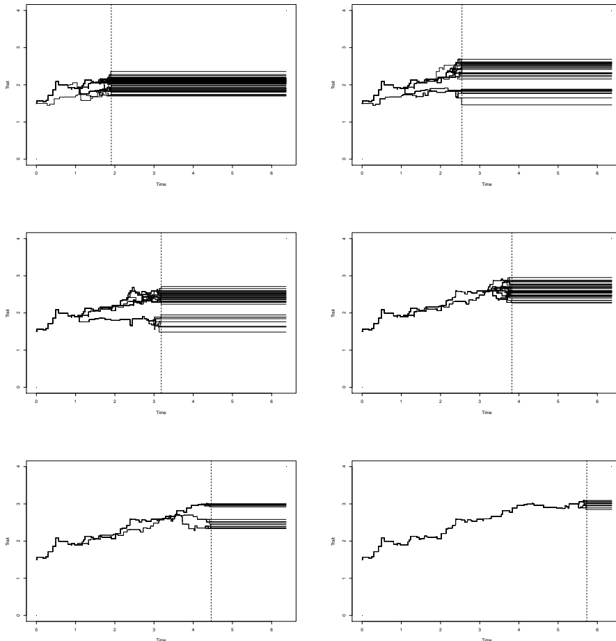
Figure 4: Kisdi's model . \alpha = 1.2 , \beta = 4 , x_0 = 4 , \sigma = 0.2 , p = 1 , K = 2 , n = 10 . The 50 particles are started with the trait 1.5.
