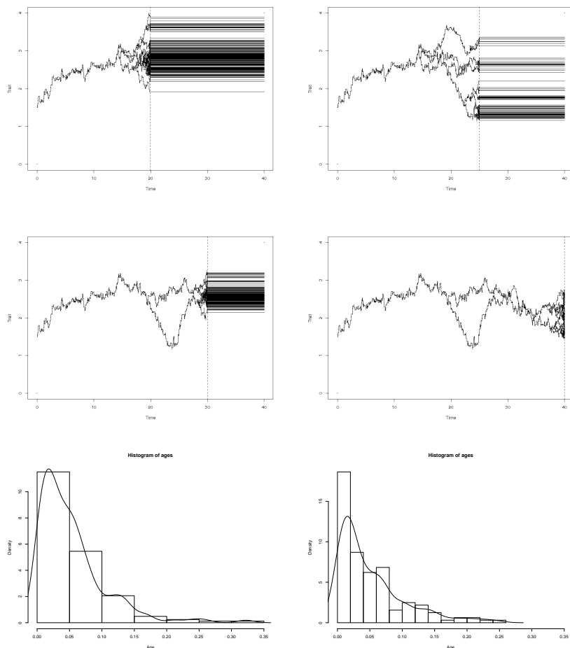
Figure 8: Simulation for the logistic age and size-structured population. The last line corresponds to the age-distribution at time t = 0.5 and t = 4 . \sigma = 0.2 , p = 1 , x_0 = 4 , d_0 = 0.25 , \eta = 0.1 , n = 20 . The 100 particles are started with trait 1.5 and age 0.
