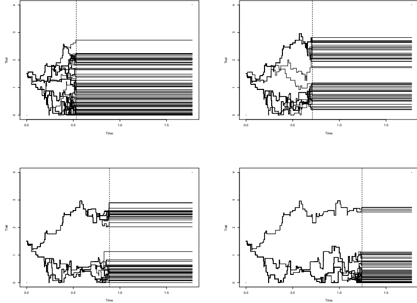
Figure 6: Simulation for Adler's fattened goats. \alpha = 10 , \varepsilon = 0.8 , b = 0.75 , \sigma = 1 , p = 1 , K = 50 and n = 50 . The 100 initial particles are started at location 1.5.
