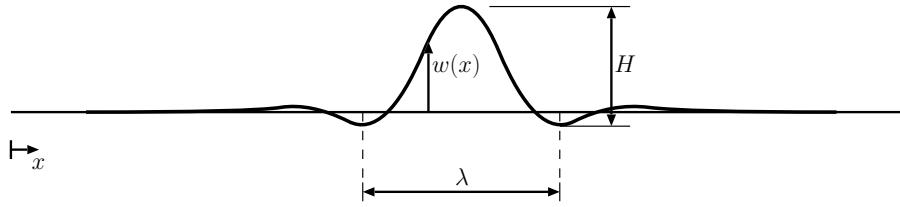
Fig. 8. Definition of localized buckle wavelength \lambda and maximum wave height H .
