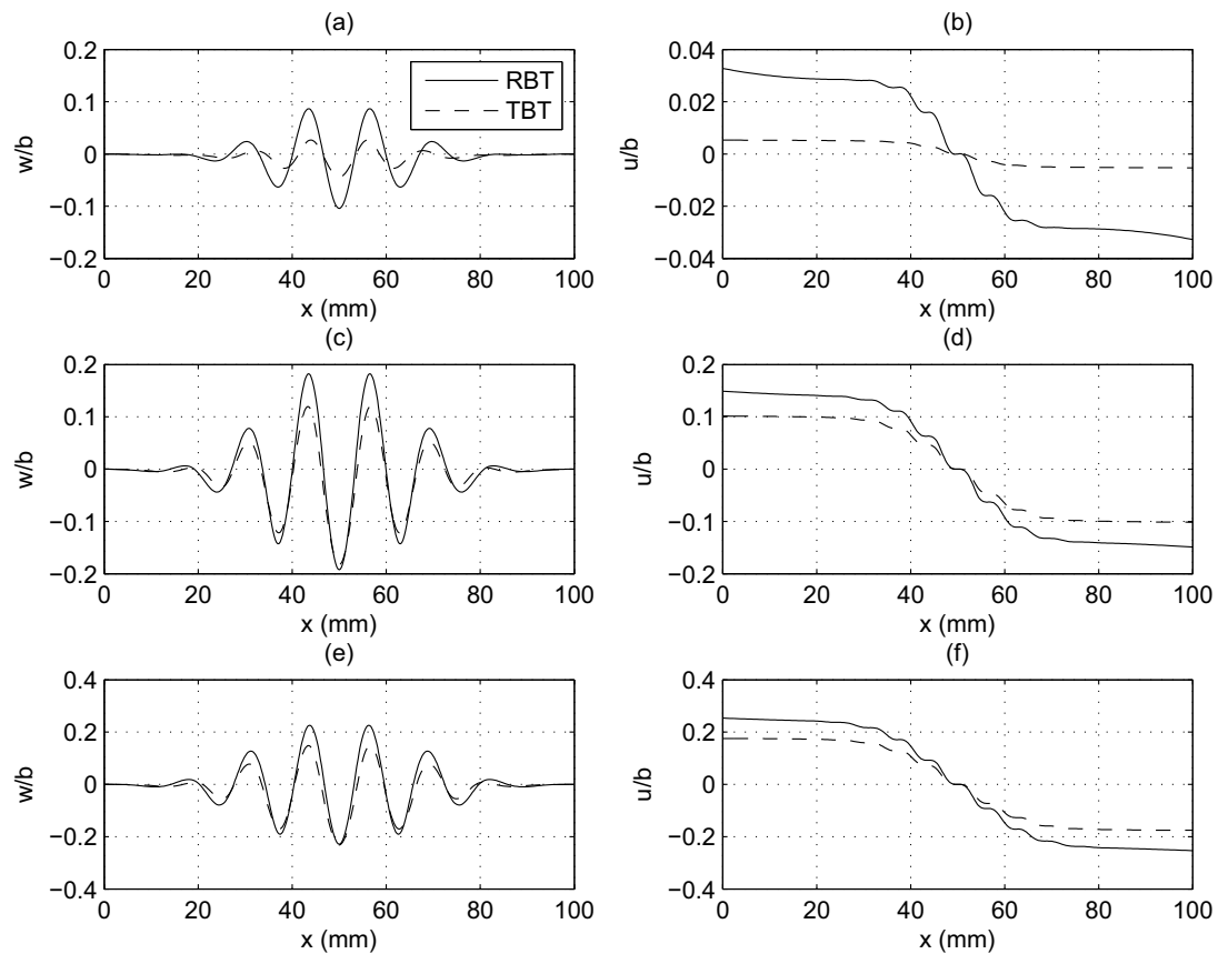
Fig. 7. The evolution of the local modes w(x) and u(x) for the two modes for different stages in the unloading path (a)–(b) P/P^C = 0.9 , (c)–(d) P/P^C = 0.7 and (e)–(f) P/P^C = 0.6 . In this case: L = 100 mm and b = 5.08 mm.
