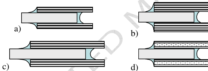
Fig. 7- a) Al (3.2)-[0°] 8 (1.6) L 0 =12.5mm, b) Al (3.2)-[0°] 16 (2.9) L 0 =12.5mm, c) Al (3.2)-[0°] 12 (2.2) L 0 =20mm, d) Al (3.2)-[0° 2 ,90° 2 ] s (2.2) L 0 =12.5mm.
