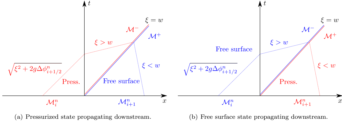
Figure 9: Full Kinetic Approach for the case of a transition point.
