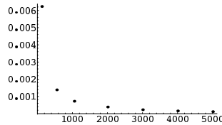
FIG. 1: Difference between the equilateral \{6j\} -symbol and the analytical result (24). The x-axis stands for l = d/2 and d goes from 100 to 5000. The error decreases as expected as l^{-1} confirming our asymptotic formula.
