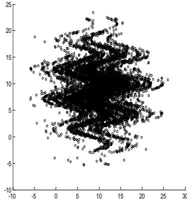
Fig. 1 Chaotic multifold attractor of the map (1) obtained for a = 4 and b = 0.9 .
