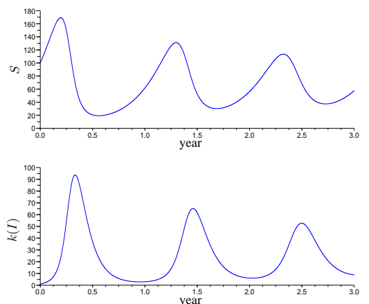
Fig. 3. Scenario 3, S(t) and k(I)(t) on 3 years
