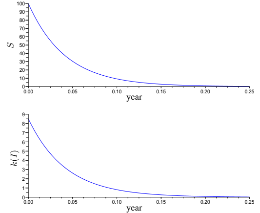
Fig. 2. Scenario 2, S(t) and k(I)(t) on a quarter of year
