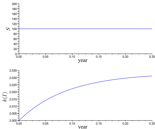
Fig. 1. Scenario 1, S(t) and k(I)(t) on a quarter of year
