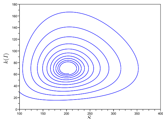
Fig. 4. Scenario 3, phase-plane (S, k(I)) on 10 years
