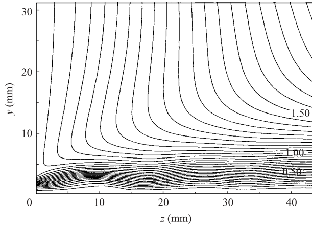
FIGURE 12. Streamline picture of the flow behind the nozzle under conditions of Exp. #3.
