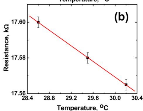
Figure 20. Resistance versus temperature measurement for (a) double \beta -SiC NW, which has -10^\circ\text{C}^{-1} and (b) single \beta -SiC NW, which has -22^\circ\text{C}^{-1} . (Reproduced with permission [66] ©IOP 2010).
