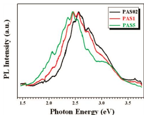
Figure 17. Photoluminescence spectra of 6H-SiC nanowires recorded from different samples with increasing Al concentration (PAS02<PAS1<PA05). (Reproduced with permission [43]. © American Institute of Physics)
