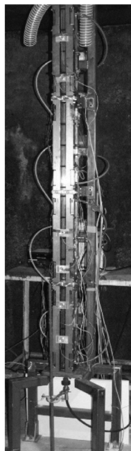
Figure 2. Global view of experimental set-up. [Color figure can be viewed in the online issue, which is available at www.interscience.wiley.com .]
