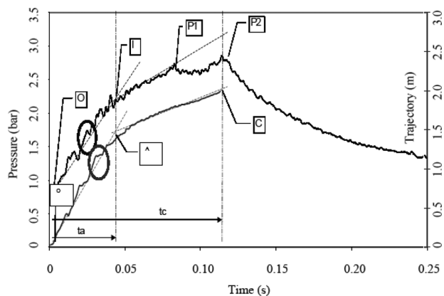
Figure 9. Pressure signal and flame trajectory.
