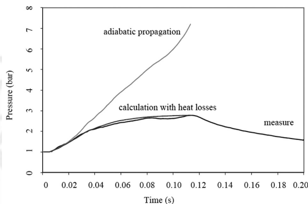
Figure 7. Pressure versus time.
