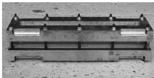
Figure 3. One part of the tube and its metallic skeleton. [Color figure can be viewed in the online issue, which is available at www.interscience.wiley.com .]
