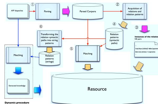
Fig. 1 Framework for ontology enrichment
