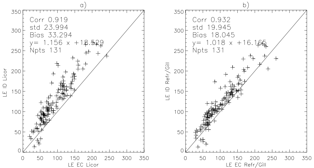
Figure 15. Comparison of EC and ID latent heat fluxes. (a) Data from the Licor and (b) refractometer data.
