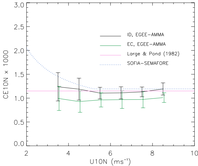
Figure 18. Neutral 10 m Dalton number as a function of 10 m neutral wind. The vertical bars denote the standard deviation of CE10N.
