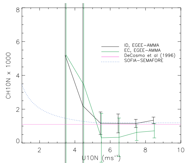
Figure 17. Neutral 10 m Stanton number as a function of 10 m neutral wind. The vertical bars denote the standard deviation of CH_{10N} .
