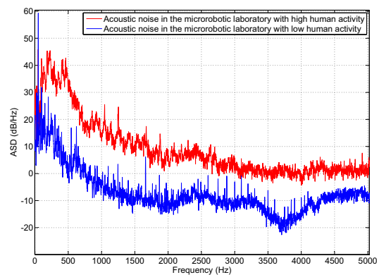
Fig. 4. ASD of acoustic noises within the microrobotic laboratory.
