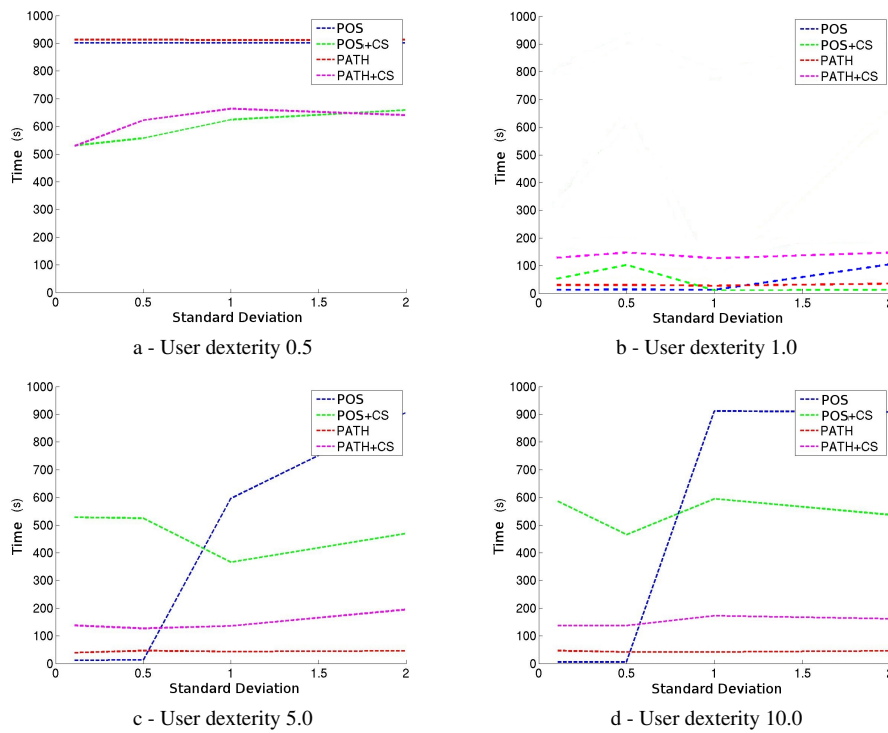
Fig. 17 Comparing the sampling method effect on resolution time given the standard deviation for different user dexterity values.
