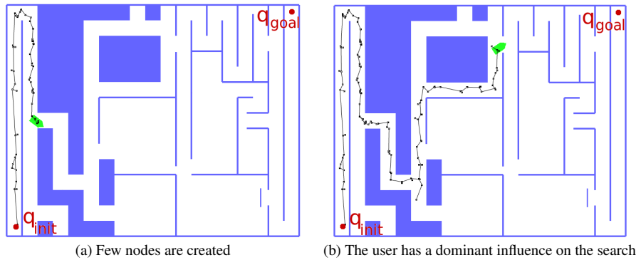
Fig. 7 The user is leading the search and the algorithm is tracking his position
