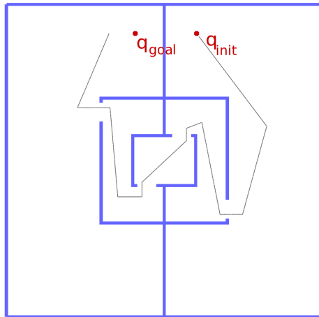
Fig. 14 Testing environment. The user's path is displayed in black.
