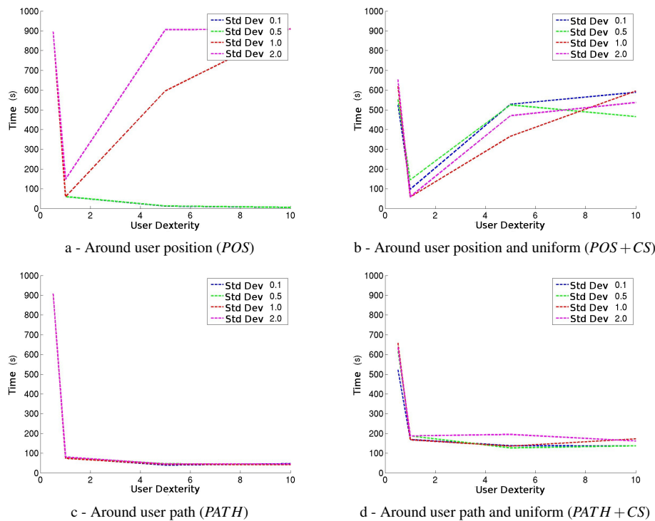
Fig. 15 Comparing the standard deviation effect on resolution time given the user speed for different sampling methods.
