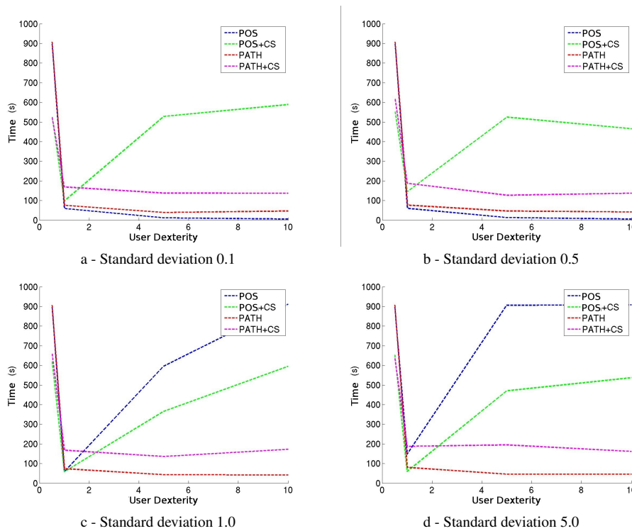
Fig. 16 Comparing the sampling method effect on resolution time given the user dexterity for different standard deviation values.
