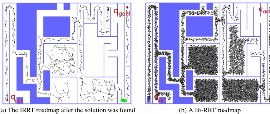
Fig. 9 Comparison between the roadmap obtained after using the IRRT algorithm and after using a Bi-directional RRT algorithm
