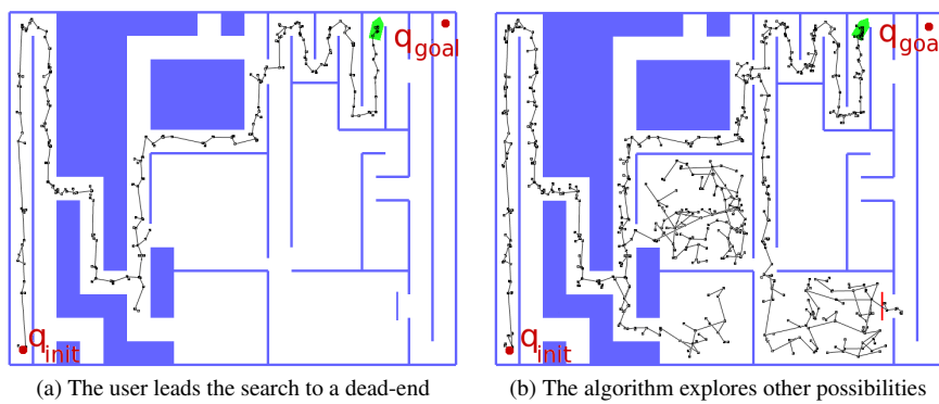
Fig. 8 The user is stuck in a dead-end, the algorithm is searching other possibilities to reach the goal
