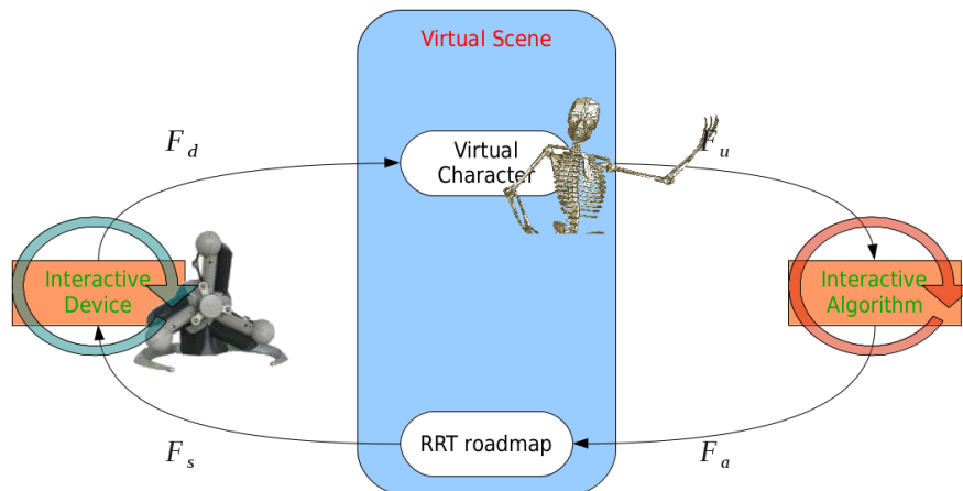
Fig. 3 General interaction loop between the algorithm and the user (represented by the interactive device) through the virtual scene
