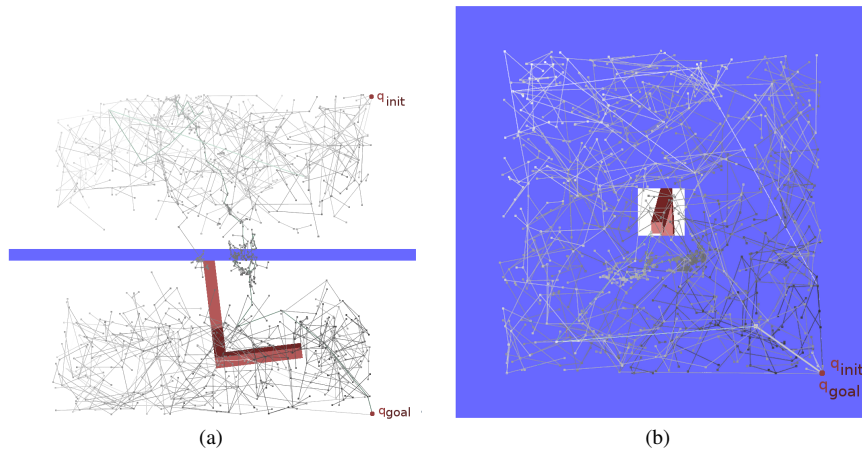
Fig. 11 The roadmap is developed on both sides of the wall
