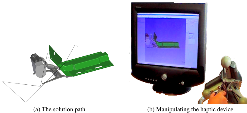
Fig. 13 Extracting the silencer using an interactive device and The IRRT algorithm
