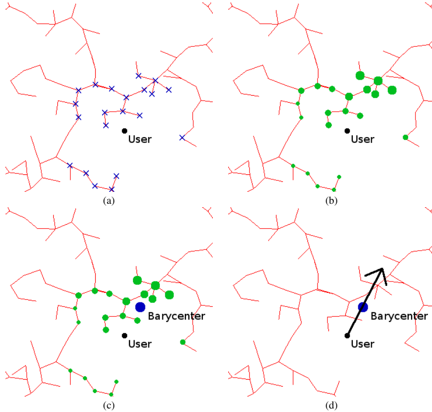
Fig. 5 Computing F_a pseudo-force.
