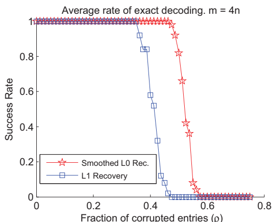
Fig. 3. Average rate of exact decoding for the case of m = 4n and n = 100 . Smoothed \ell^0 -norm recovery's parameters are set as: \sigma_{\text{target}} = 0.0001 , \kappa = 0.87 , L = 3 and \mu_0 = 2 .
