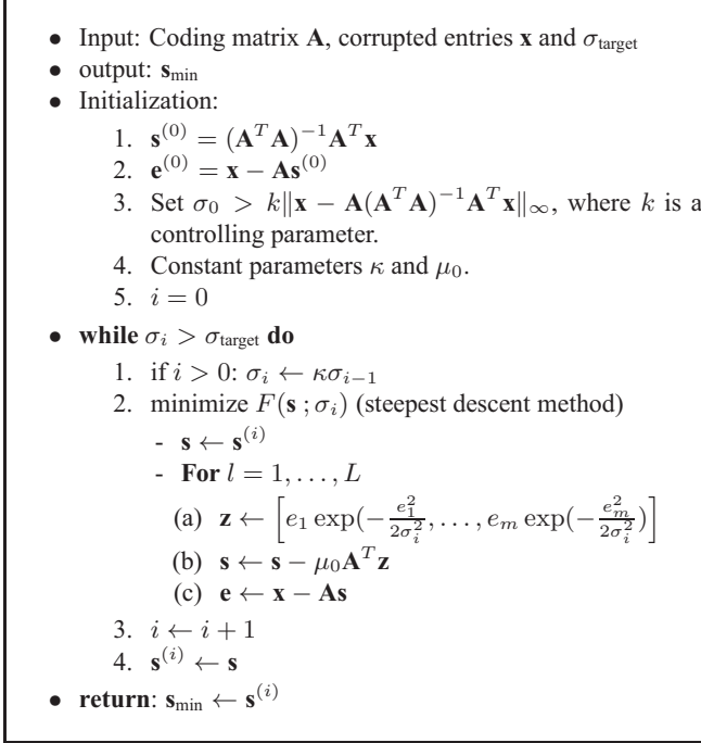
Fig. 1. Smoothed \ell^0 -norm recovery algorithm.
