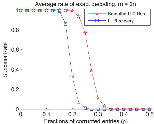
Fig. 2. Average rate of exact decoding for the case of m = 2n and n = 100 . Smoothed \ell^0 -norm recovery's parameters are set as: \sigma_{\text{target}} = 0.0001 , \kappa = 0.82 , L = 3 and \mu_0 = 2 .
