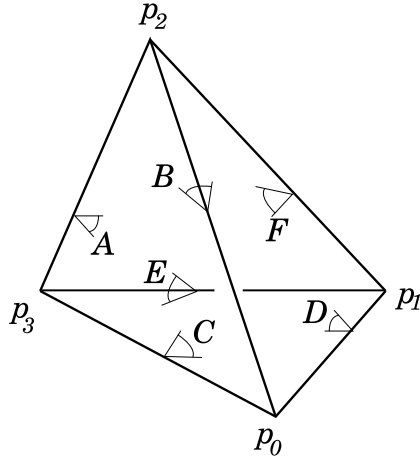
Figure 1: Spherical tetrahedron
