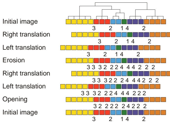
Figure 11: Erosion and opening by a segment of 3 pixels: intermediate steps
