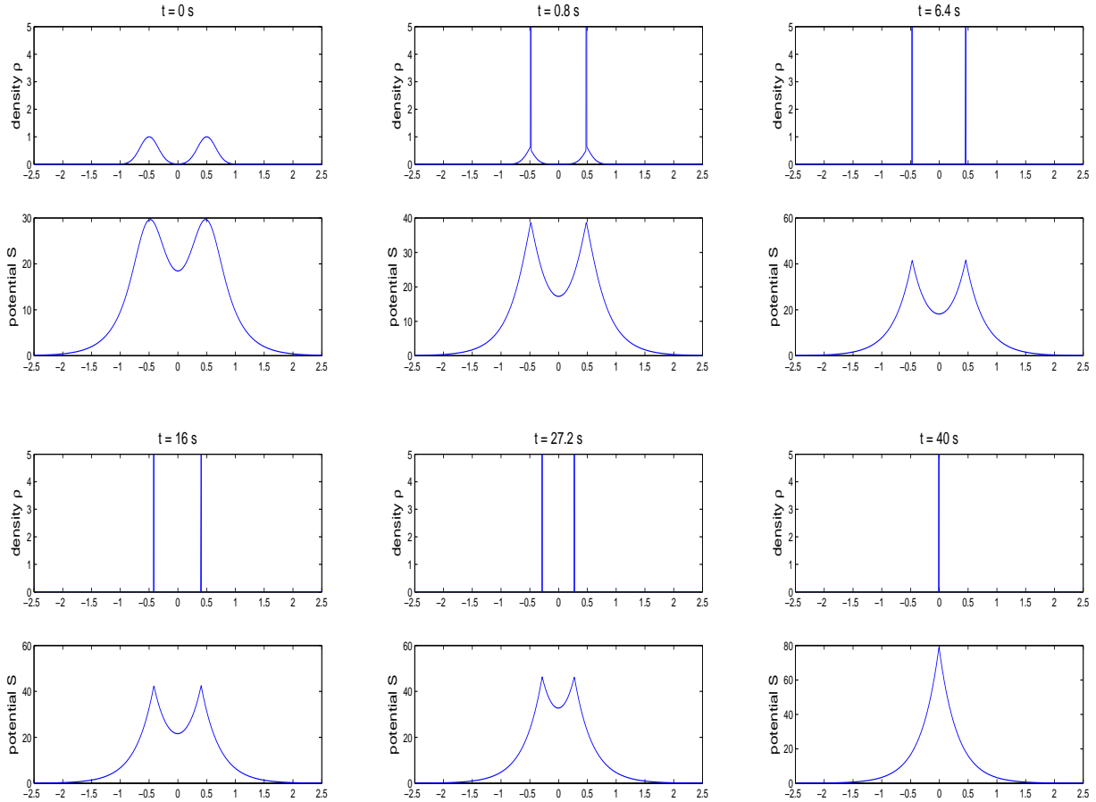
Figure 1: Dynamics of the density \rho and of the potential S for an initial density given by the sum of two Gaussian.
