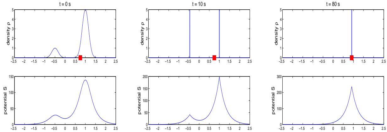
Figure 3: Dynamics of the density \rho and of the potential S with the dynamics of the center of mass represented by a red square. The center of mass moves.
