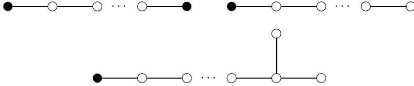
FIGURE 1. Dual graphs when \Delta \neq 0
